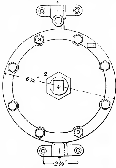
Fig. 3117. Elevation. REGULATOR.
